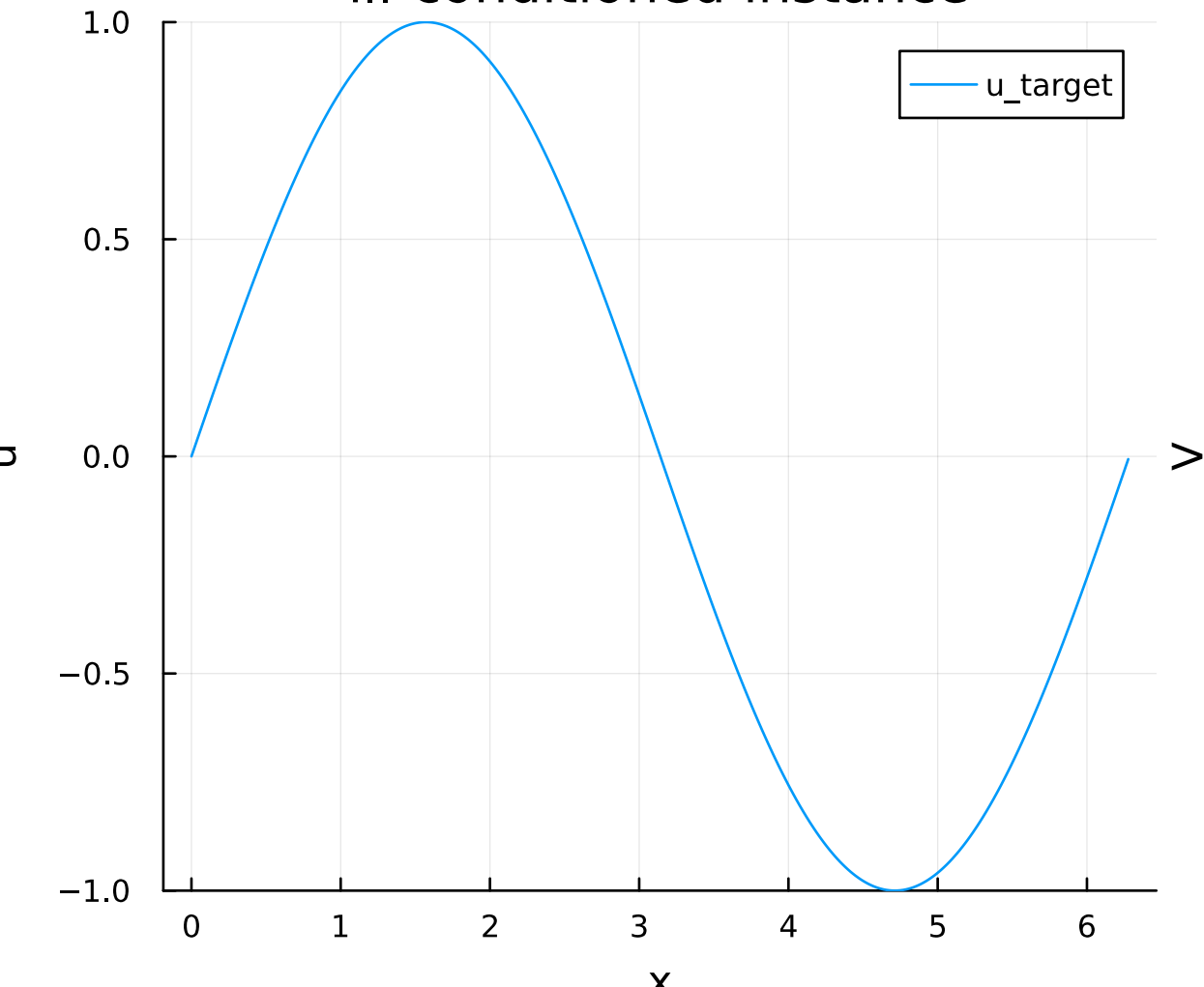
ill-conditioned instance
