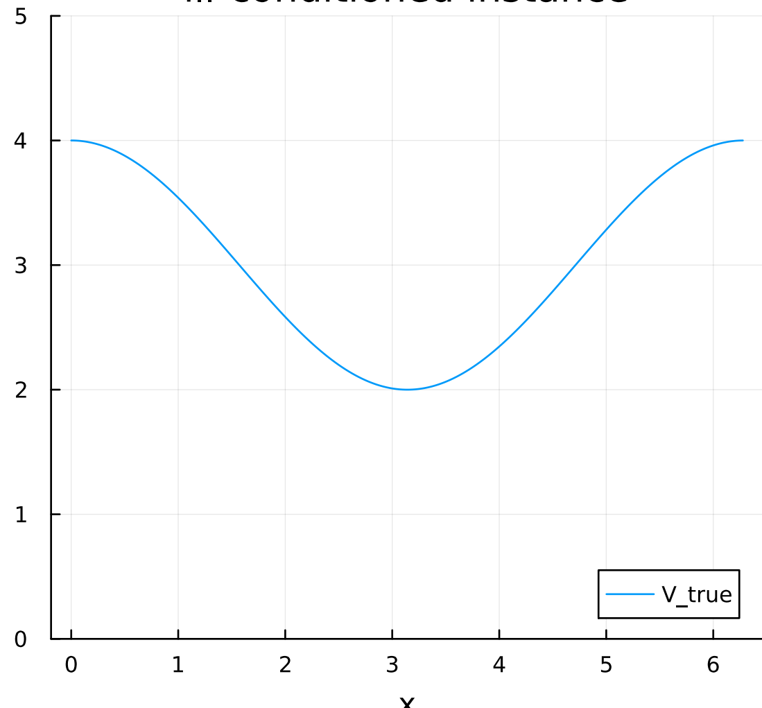
ill-conditioned instance
